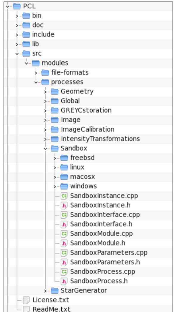
Figure 4— The Sandbox module in the PCL distribution tree.
