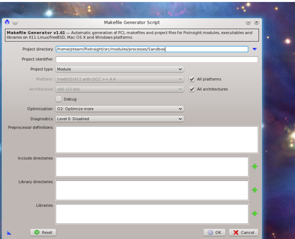
Figure 5— The Makefile Generator script.
