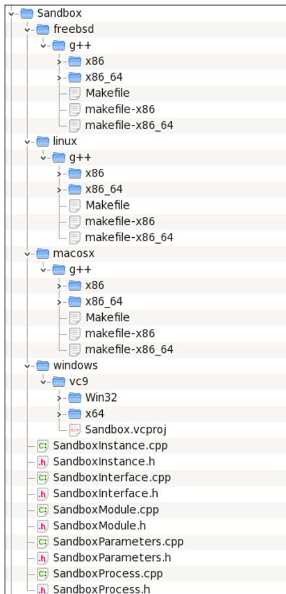
Figure 6— Makefiles for the Sandbox module.
