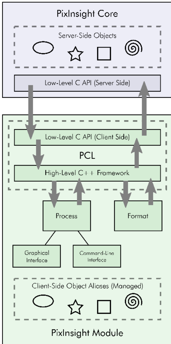
Figure 1— The modular architecture of PixInsight.
